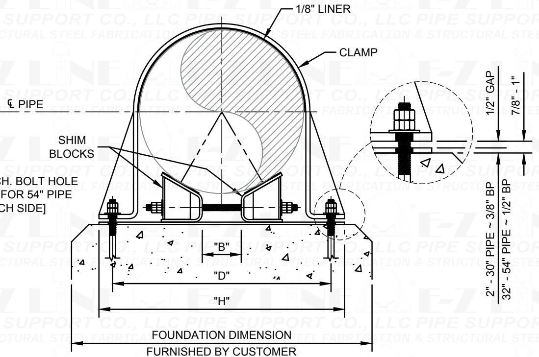
SECTION THRU PIPE AT SUPPORT
