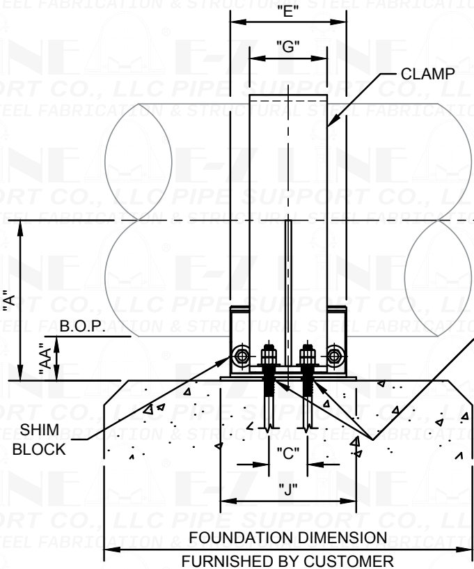
ELEVATION AT PIPE SUPPORT
