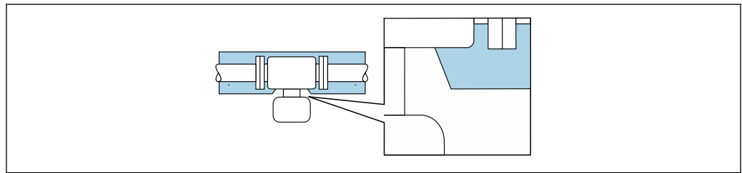
38 Thermal insulation with exposed extended neck
