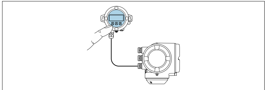
51 Operation via remote display and operating module DKX001
