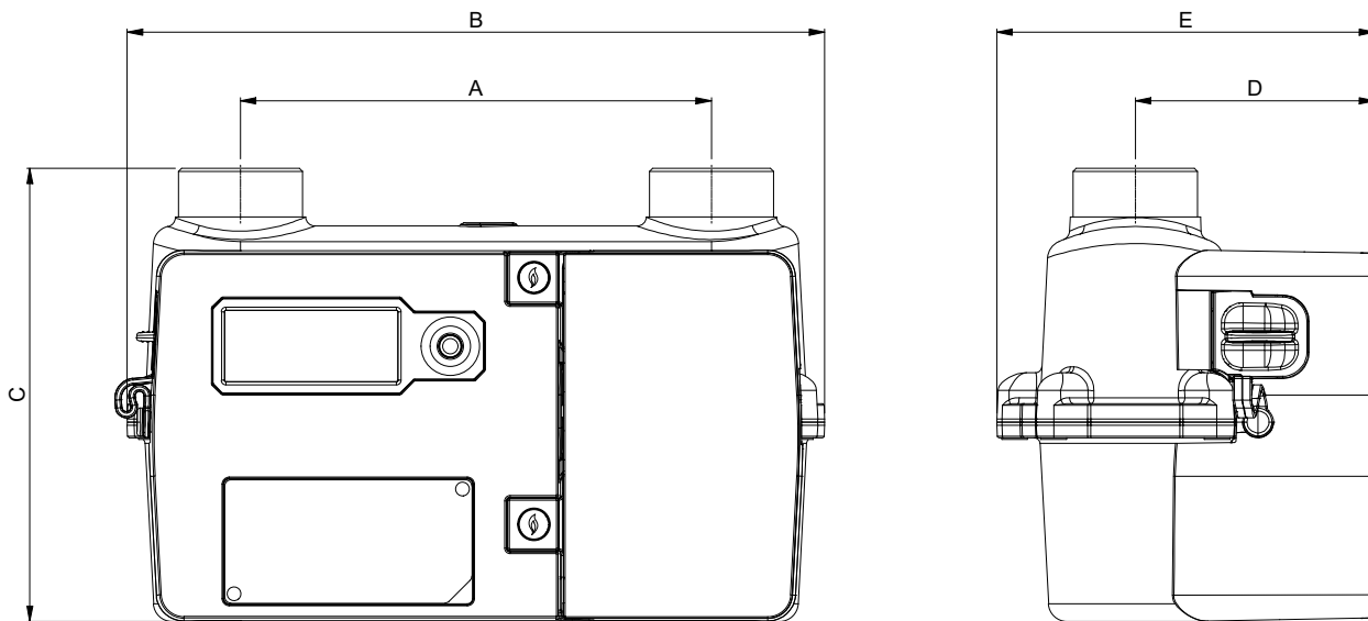
Figure 6 SSM-iCON 250 dimensions
