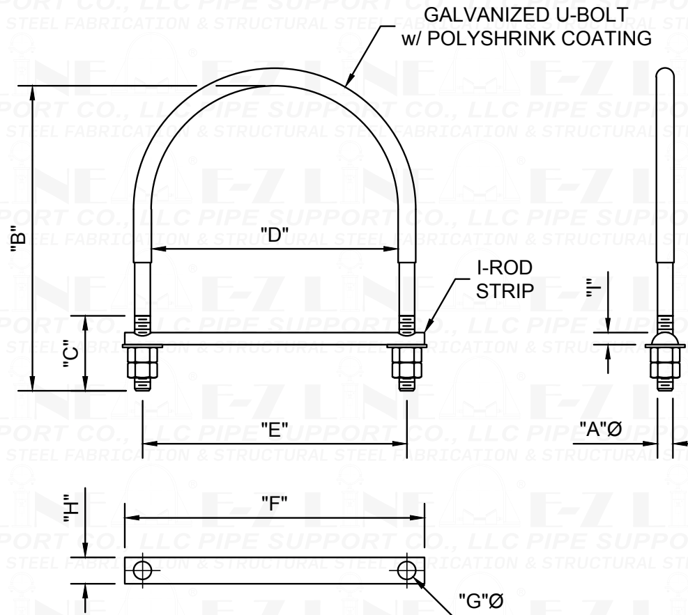
U-BOLT WITH I-ROD STRIP
