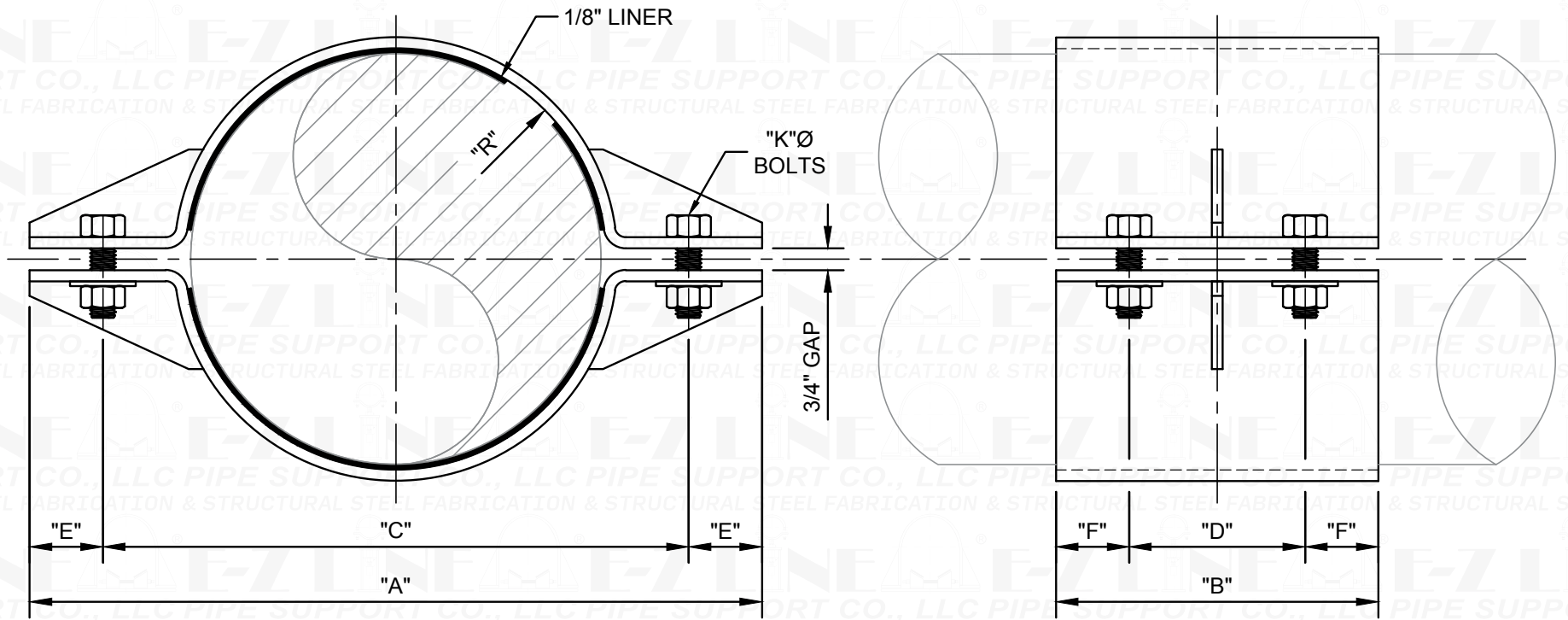
SECTION THRU PIPE AT SUPPORT
