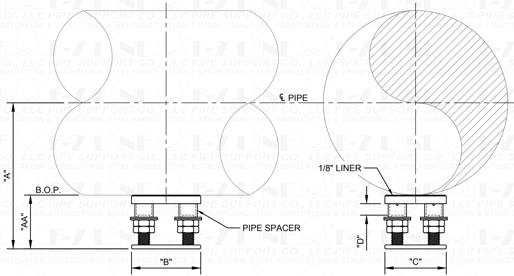
ELEVATION AT PIPE SUPPORT
