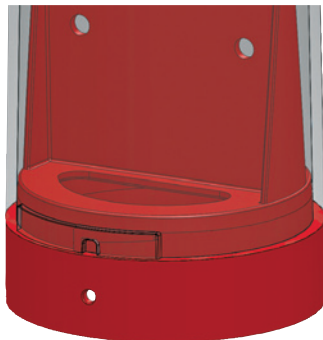
Rivets (2 supplied) hold Test Station to post.
