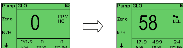
Figure 80: Bump Test - Applying Gas
