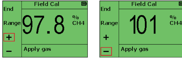
Figure 88: Field Calibration - Adjustment
