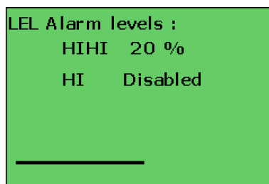
Figure 17: Warm-up - Alarm set-points (LEL)
