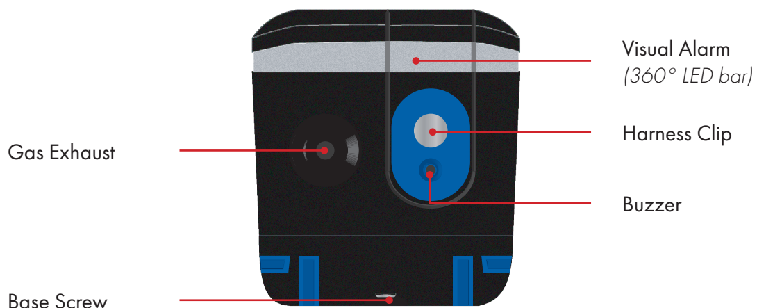
Figure 2: GS700 - Left View
