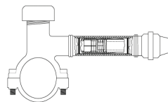
Model 65 – Mechanical tee with Model 35 attached
