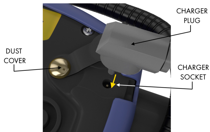
Figure 59: Connect Charger to Monitor
