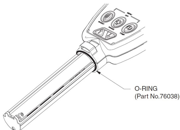
Figure 55: O-Ring Replacement
